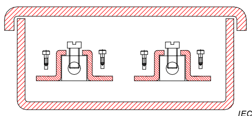
Figure AA.1c – Enclosures with provisions for subsequent incorporation of terminals or connecting devices according to 7.101.3
